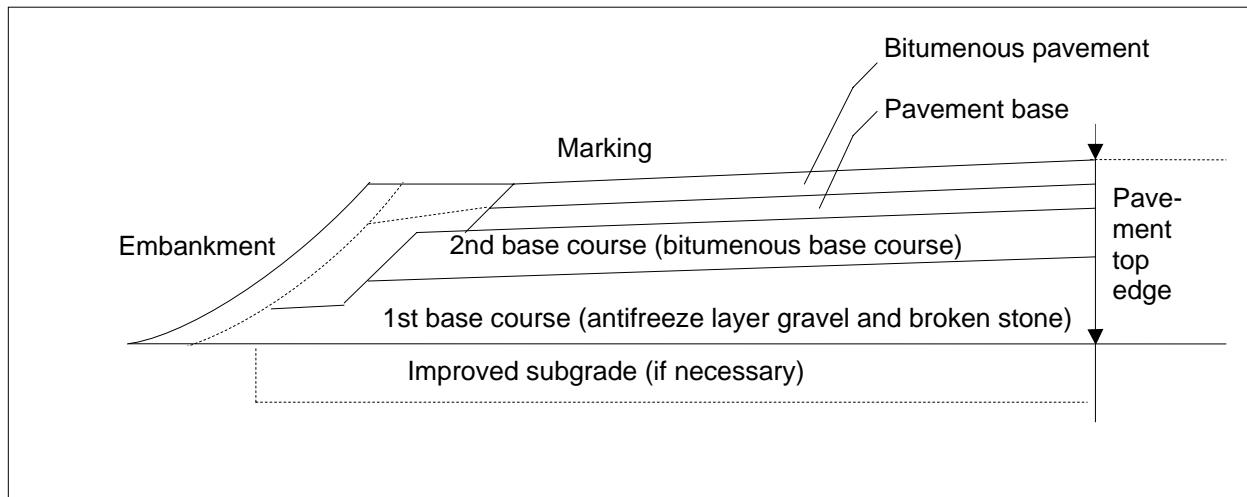
Fig. 1: Standard structure
