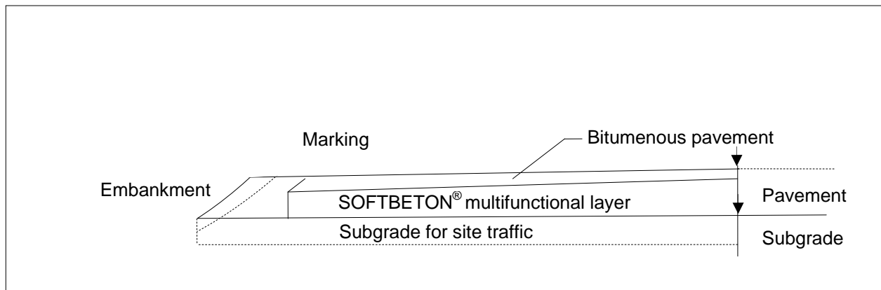
Fig. 2 SOFTBETON® structure
